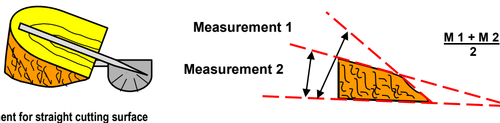
Fig. 13: Measuring the sink for straight and round cuts
